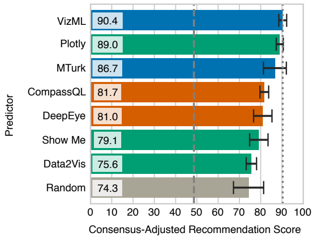
(a) Two-type (bar/line) visualization type CARS.
