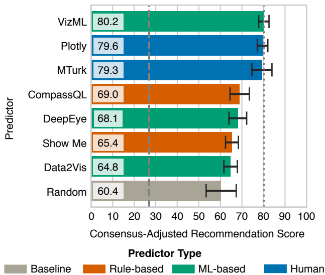
(b) Three-type (bar/line/scatter) visualization type CARS.
