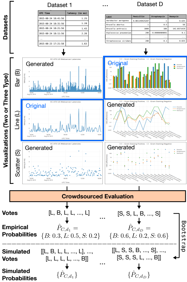
Figure S6: Experiment flow. The original user-generated visualizations are highlighted in blue, while we generated the visualizations of the remaining types. After crowdsourced evaluation, we have a set of votes for the best visualization type of that dataset. We calculate confidence intervals for model scores through bootstrapping.
