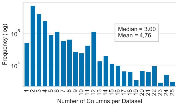
(a) Distribution of columns per dataset, after removing the 5.03% of datasets with more than 25 columns, visualized on a log-linear scale.
