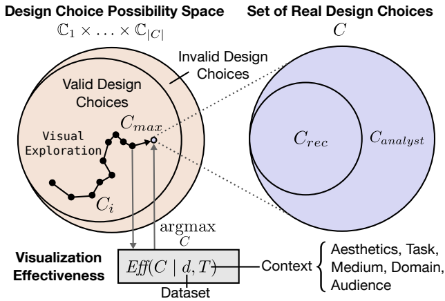
Figure S1: Creating visualizations is a process of making design choices, which can be recommended by a system or specified by an analyst.
