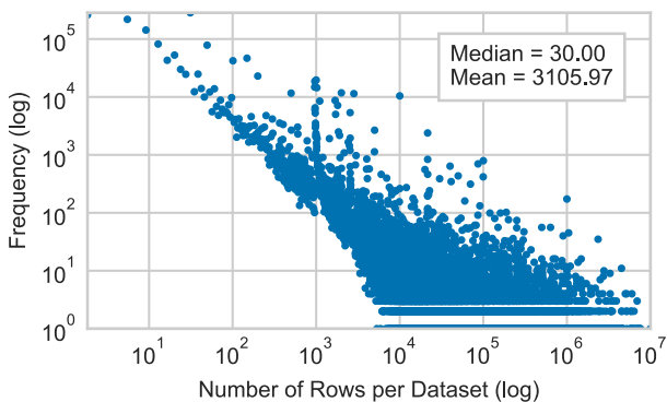
(b) Distribution of rows per dataset, visualized on a log-log scale.
