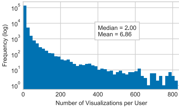
Figure S3: Distribution of plots per user, visualized on a log-linear scale.
